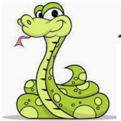
SERP
